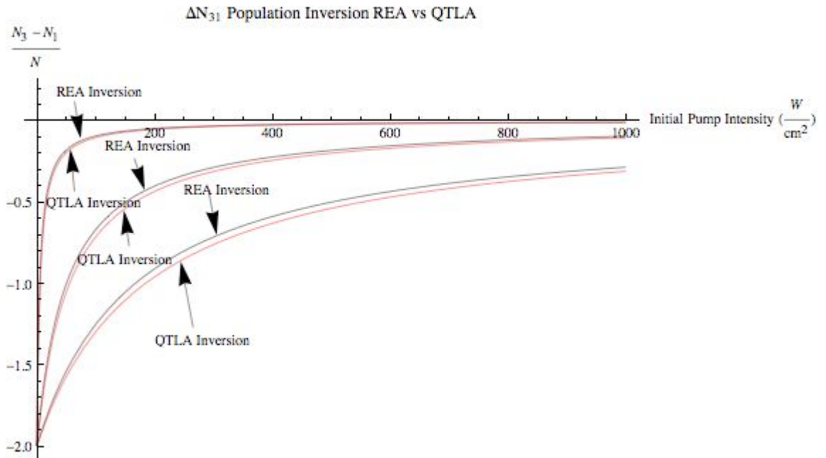
Figure 43. Normalized Population Inversions of REA model vs QTLA model at system pressure of 400, 6000, and 20000 torr.
