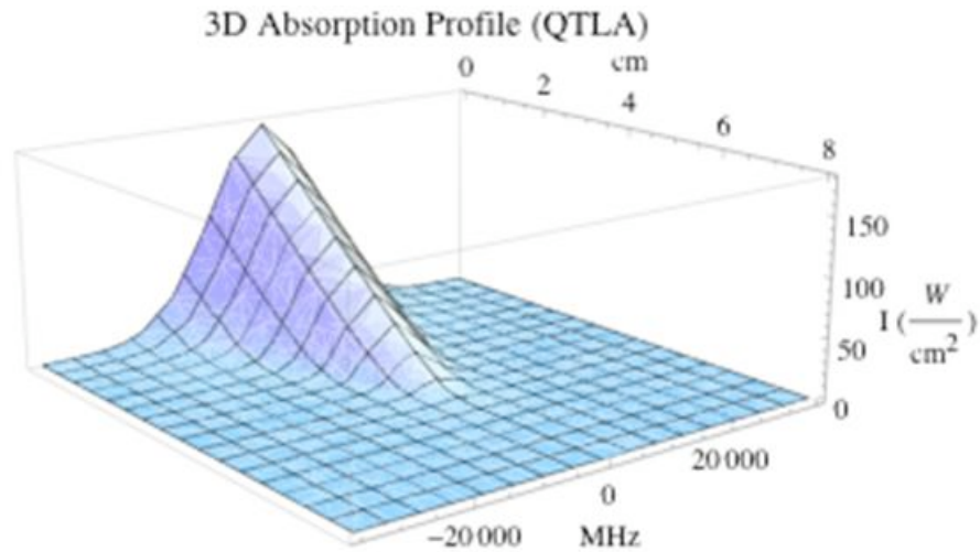
Figure 30. QTLA Profile
